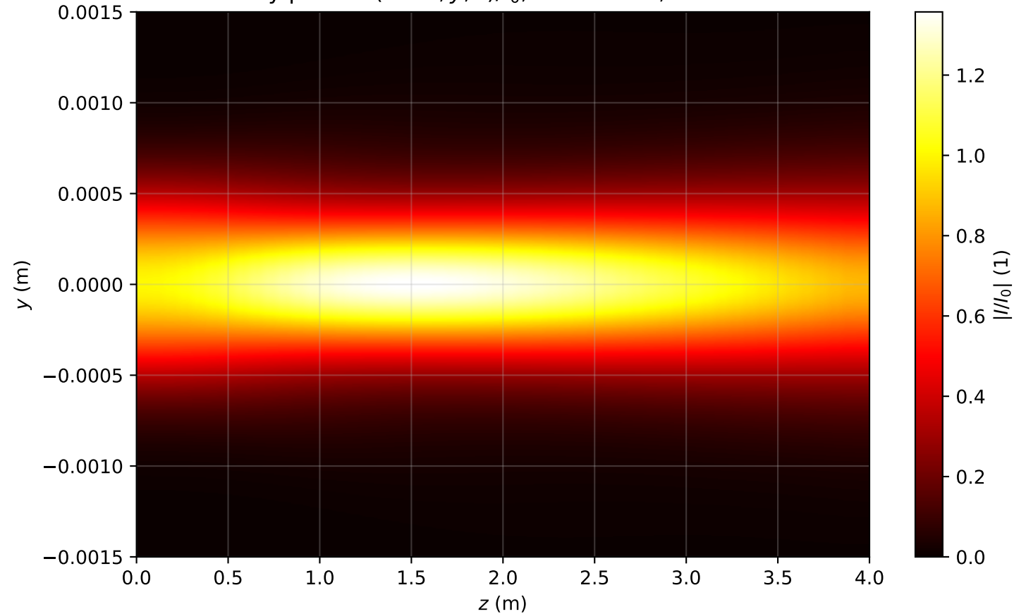
Intensity profile I(x=0, y, z)/I_0 , P_{in}=0.8P_{cr} , artificial time
